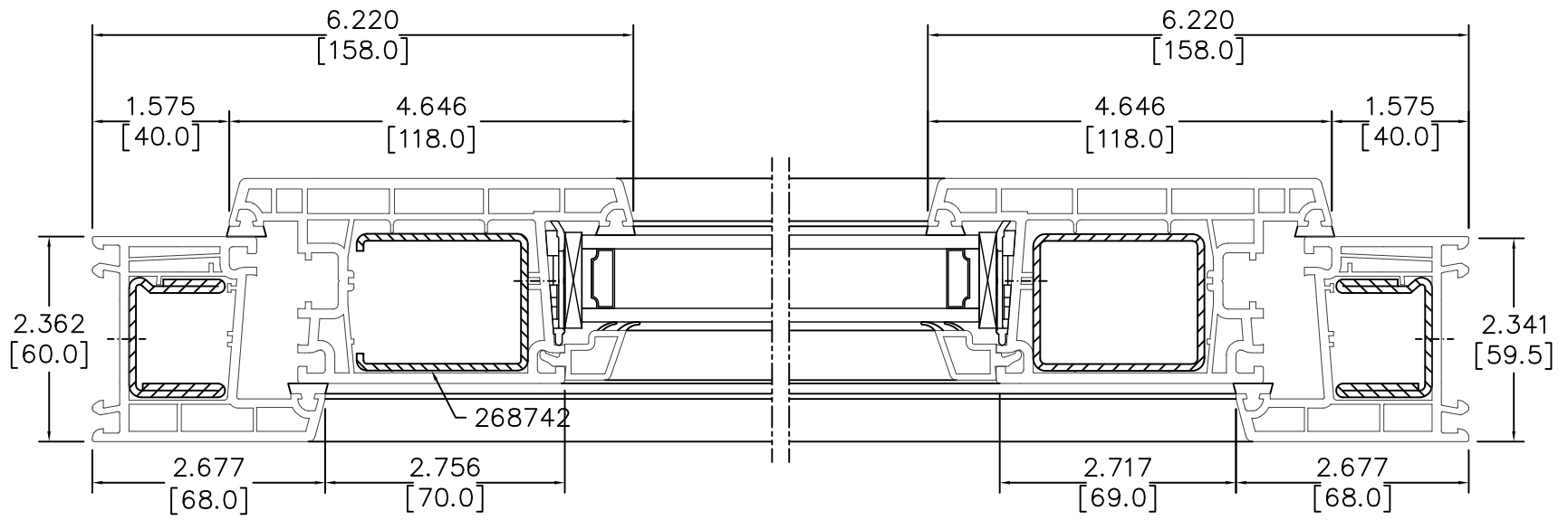
Section: B-B
