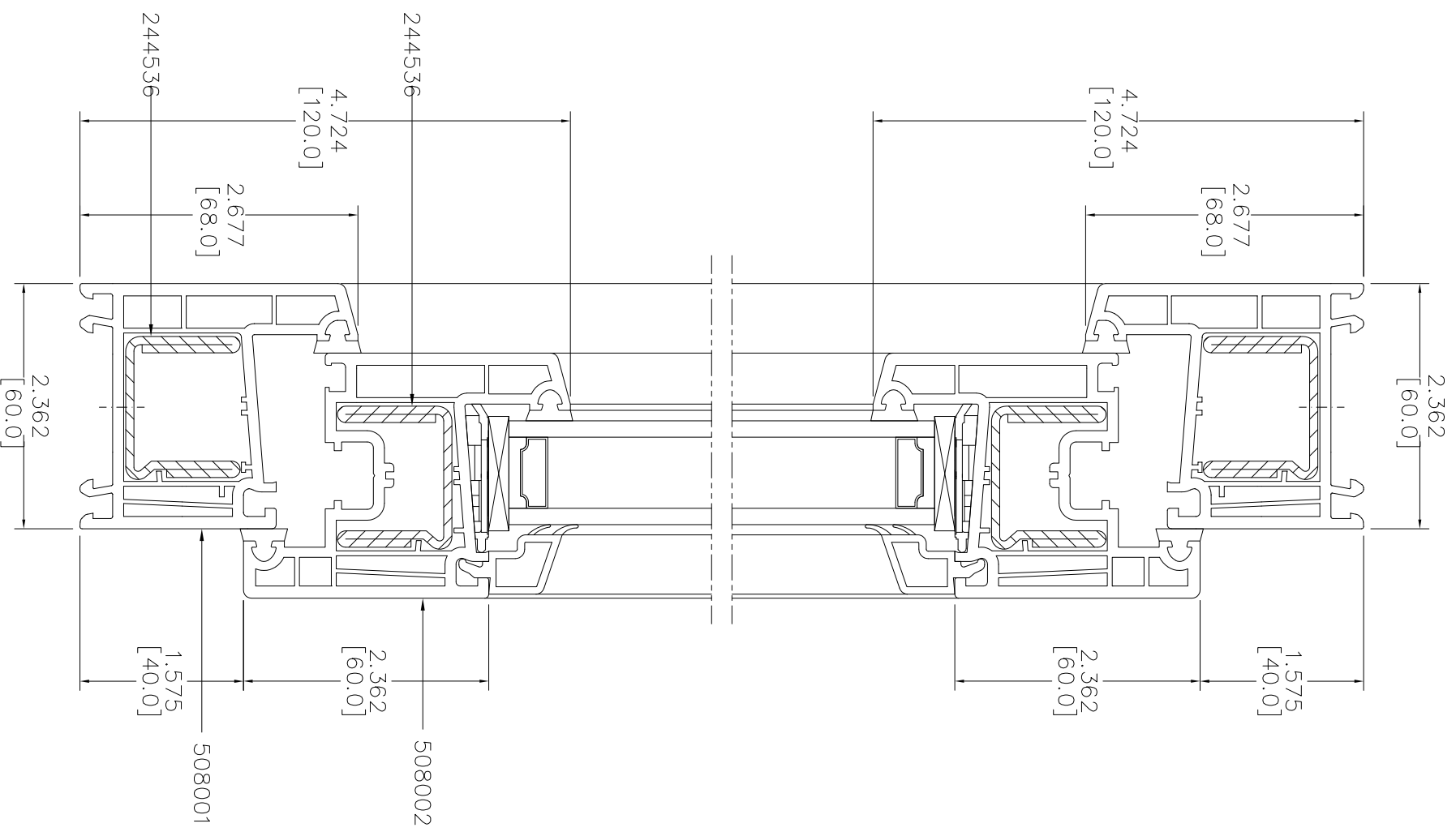
Section: A—A
