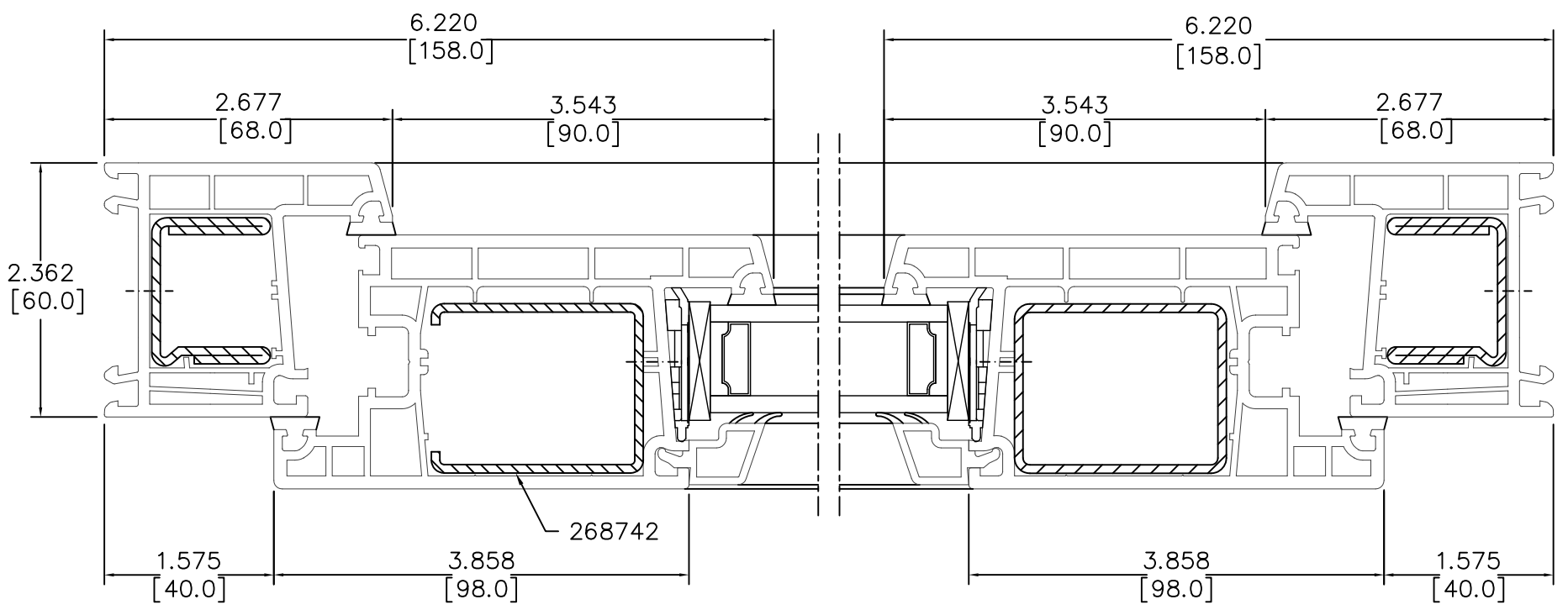
Section: B-B
